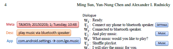
Fig. 2. Multi-app task dialog example. Meta, Desc, App were shown to the participant. Utterances were transcribed manually or via Google ASR. Apps were manually assigned to utterances.
